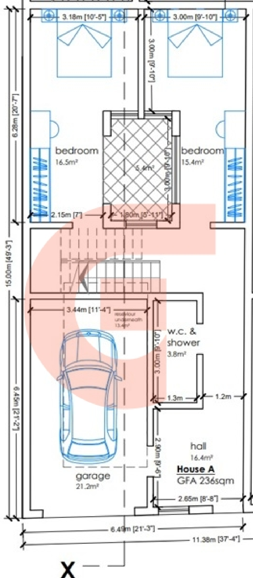
Proposed Ground Floor Level Plan Scale 1:100
